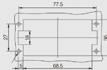
面板安装开孔图 Panel cut out
