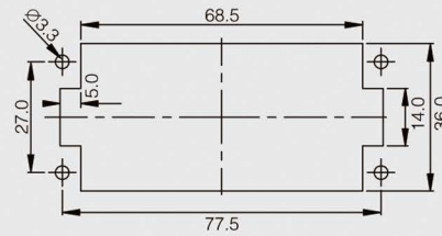
面板安装开孔图 Panel cut out
