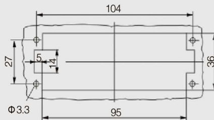
面板安装开孔图 Panel cut out
